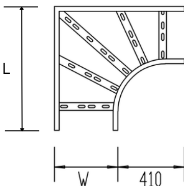
90° Horizontal Bend (90HB)
