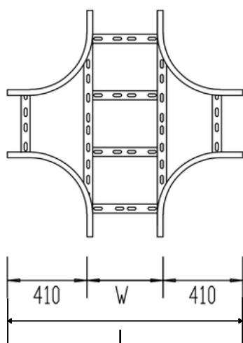
Horizontal Cross (HX)
